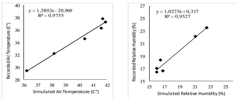
Fig. 2. Simulated and recorded values of Air temperature and Relative humidity for the current outdoor space in period time (10:00-15:00)
